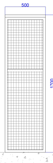
Right Side Elevation
